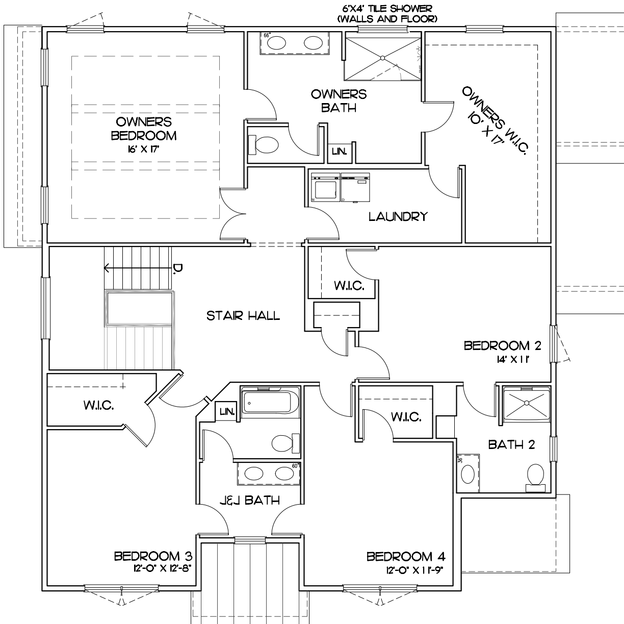
SECOND FLOOR PLAN | 1,740 S.F. | 9' CEILINGS
