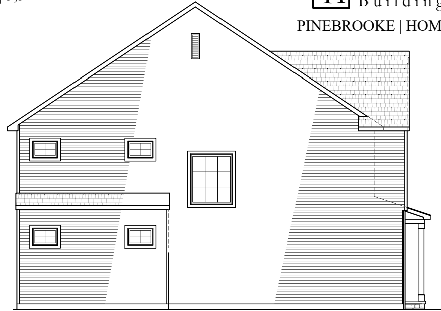
LEFT ELEVATION
