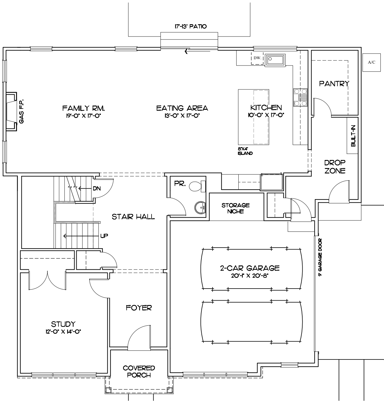
FIRST FLOOR PLAN | 1,582 S.F. | 10' CEILINGS
