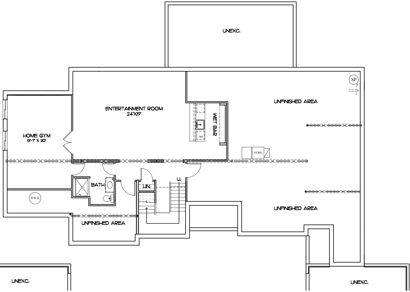
BASEMENT PLAN 10' SUPERIOR WALLS 1,198 SF FINISHED
