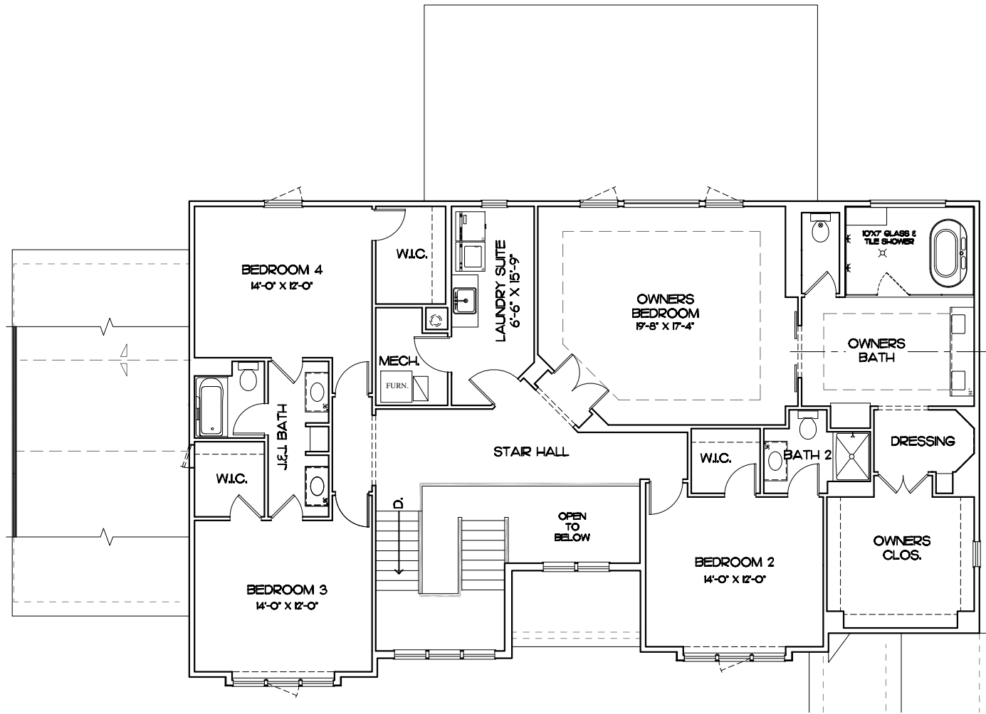
SECOND FLOOR / 1,949 SF PLAN / 9' CEILINGS
